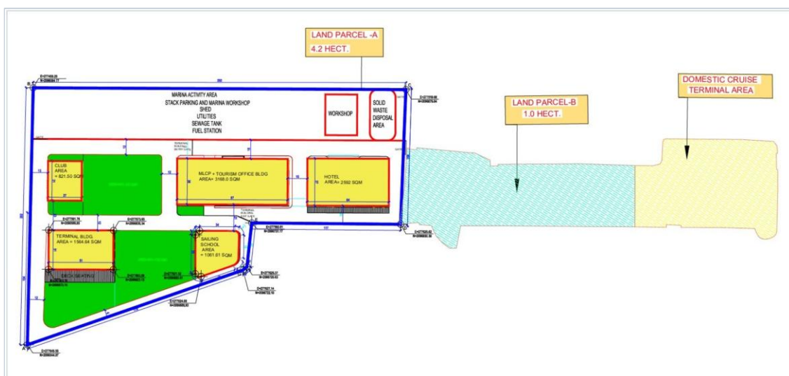
Figure 2. Proposed onshore facilities on Land Parcels A and B (indicative). Source: Draft Concession Agreement, Appendix 1.
